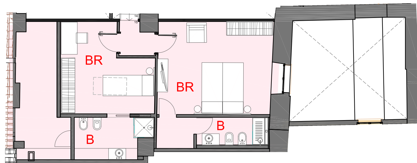
MEZZANINE
